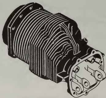
FIGURE 6-42. Cracked cylinder fins.
